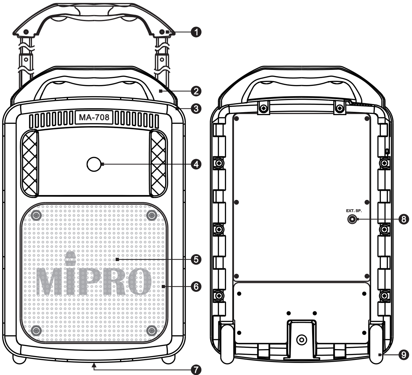
Front Panel
